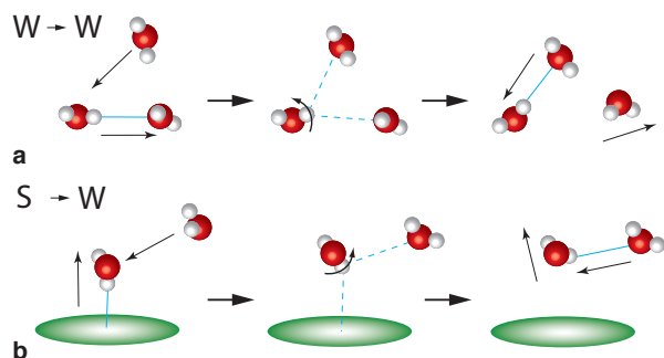
Fig. 4 Schematic illustrations of the H-bond jump exchange mechanism for (a) W T,B → W T,B and (b) S → W T jump events. Importantly, this process can be fruitfully viewed as a chemical reaction that proceeds from an initial reactant state (left) to a final product state (right) through a transition state (middle). Key molecular motions are indicated by black arrows. 16,17
